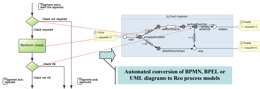
Fig. 5. Process formalization: Abstracted fragment for approval is converted to Reo
