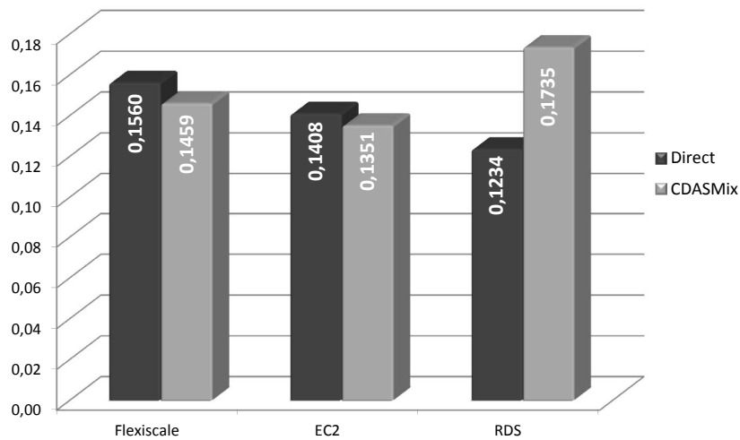
Figure 5: Average Throughput (Transactions per Second): Without (Direct) and With Using CDASMix
