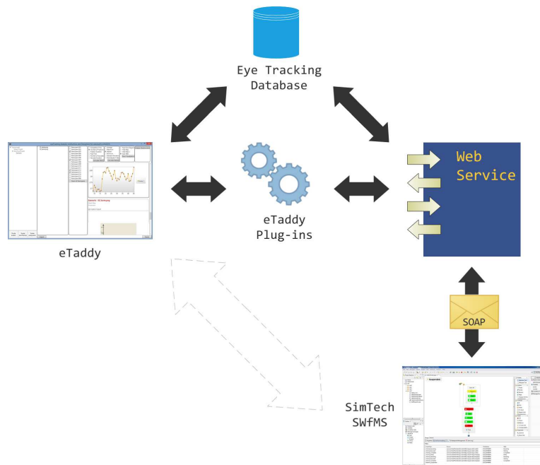
Figure 3: The functionality of eTaddy, namely the metrics, statistics, and visualizations, can be accessed through plug-ins. The eye movement data is saved in a database. A web service wrapper implementation exchanges references to the data in the database and communicates via SOAP messages with the workflow system where the eye movement analysis is modeled.
