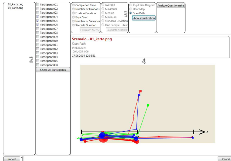
Figure 2: Eye Tracking Analysis, conDuction, and Designtool of user studYs (eTaddy) [BRE13] is a software to create eye tracking user studies, collect data, and analyze the eye movement data. For the analysis, the user has to import the eye movement data into a database (1). Afterwards, a stimulus, as well as participants can be chosen (2). Several eye tracking metrics, statistics, and visualization are available (3). The results of a calculation are shown in a timeline (4).
