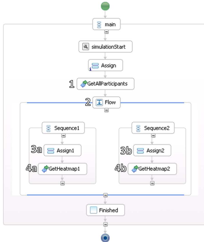
Figure 6: Example workflow calculating two attention maps for two groups of participants. First, all participants are retrieved from the database (1), then the attention maps for the two groups are created in parallel (2). On the left, the participants younger than 22 are used (3a) and then the attention map for this group is calculated (4a). Parallel to this, the participants older than 22 are used (3b) to create the second attention map (4b).
