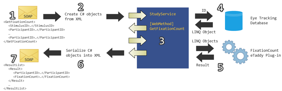
Figure 4: A workflow sends a request as a SOAP message containing the function and the necessary parameters. The parameters are cast into a C# object and sent to the web service. The web service retrieves the appropriate data from the database and calls the function. The result is then serialized into XML and sent back as a SOAP response message to the workflow.
