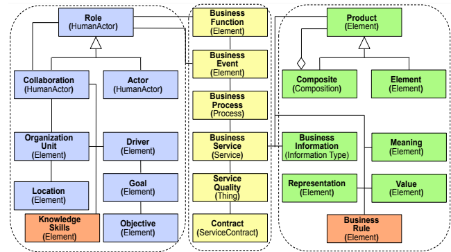
Figure 3. Ontology-supported Architecture Metamodel.
